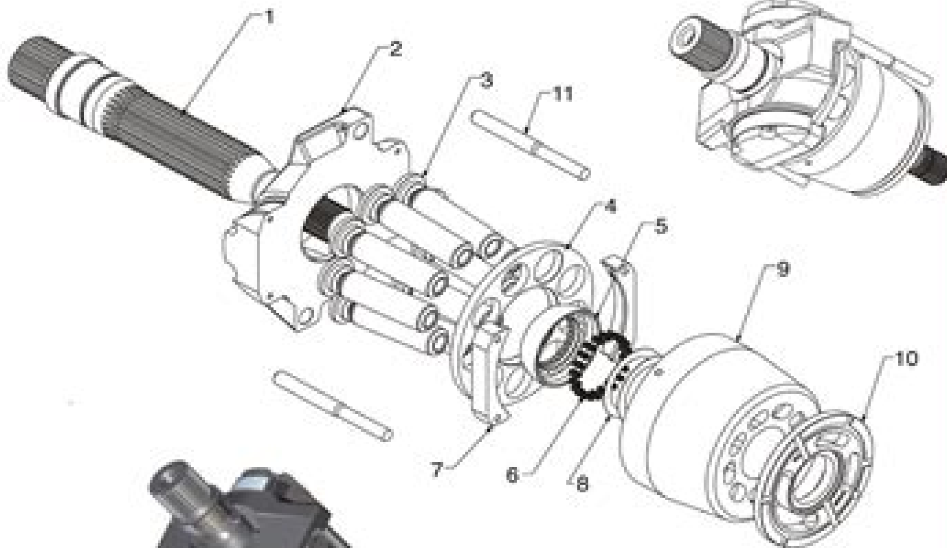
A11VSO40/60/75/95/130/145/160/190/260
