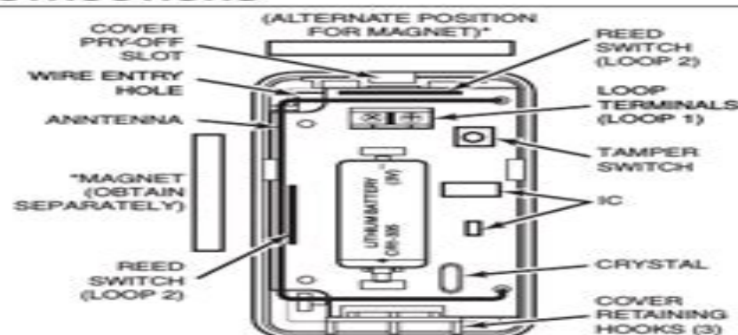
Figure 2. 5815 (shown without cover)
