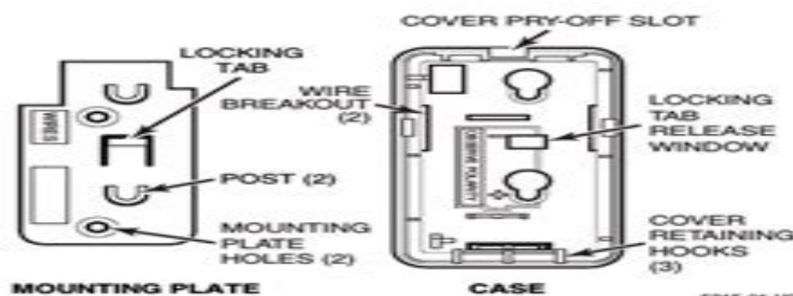
Figure 1. Mounting Plate and Case
