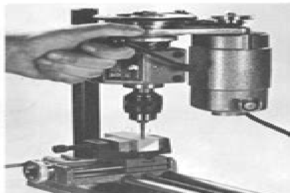
FOR DRILLING the headstock mounts on auxiliary column, lever advances spindle.
