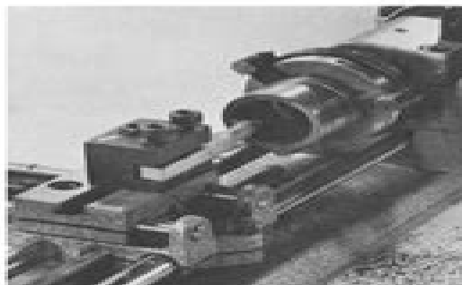
FOR BORING large holes in the lathe a boring tool is set parallel with bed.
