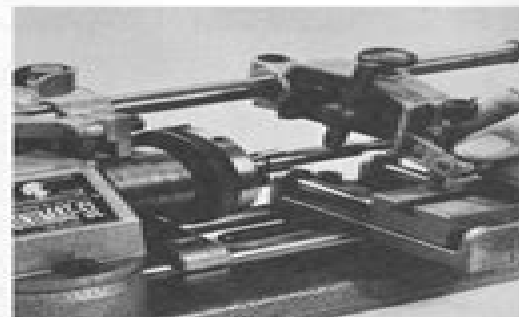
FOR THREADING a master bushing advances the threading attachment's tool bit.
