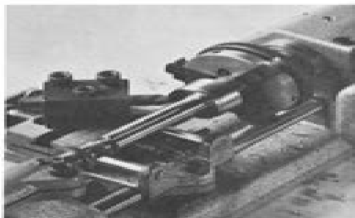
FOR METAL TURNING, lathe bit is held in tool block mounted on the carriage.
