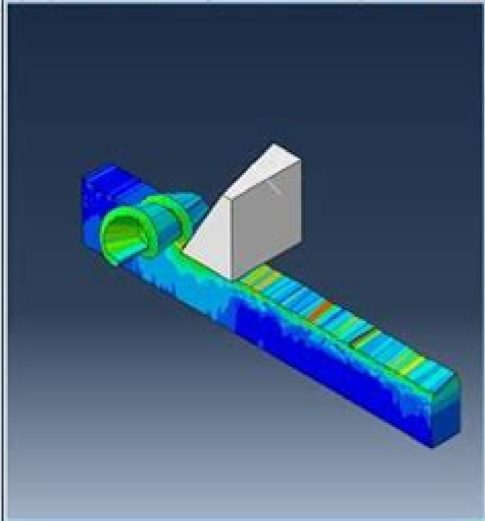
Viewport 2 009: C:\YouTube\CAE_Models\Johnson-Cook\Cooking.off
