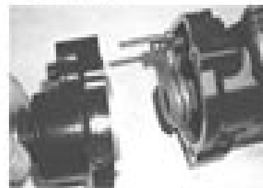
2. Using a rubber mallet, remove the bearing. Account for a gasket. Remove the lock, collar, and spring. Note the location of all the components for reassembly purposes.
