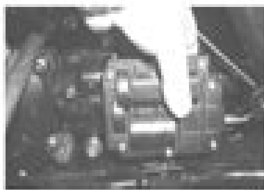
18. Remove the lower differential mounting cap screws. Account for a lock nut and washers.
