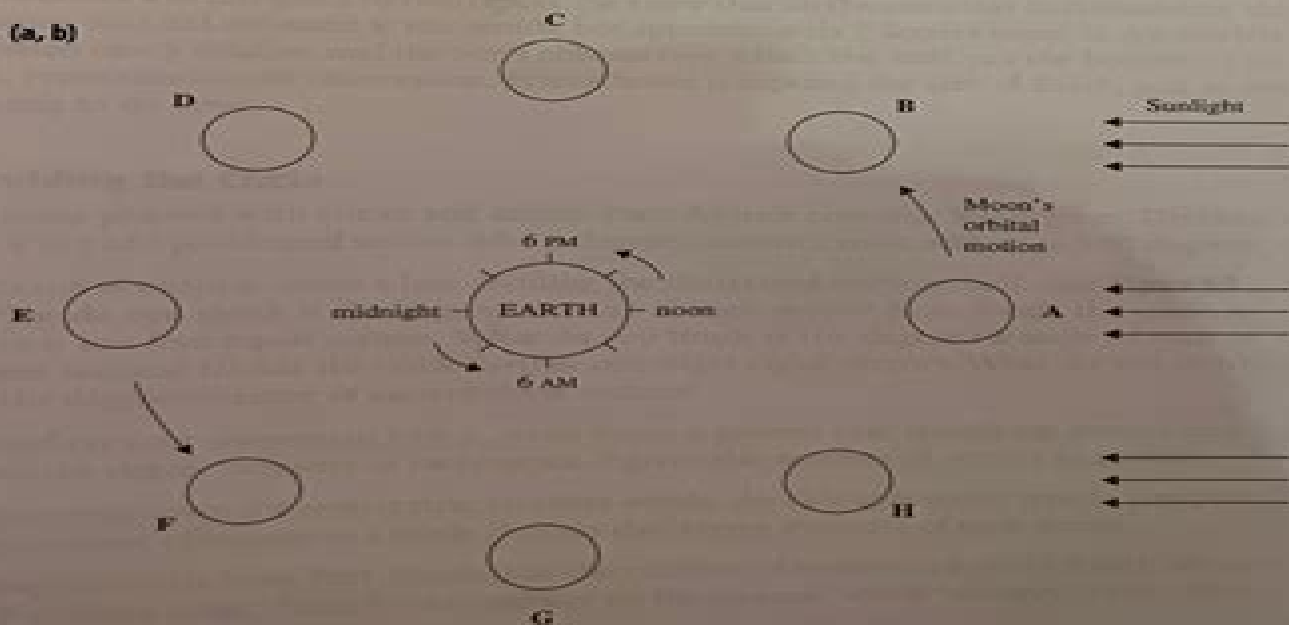
Figure 5-2 Top-down view of the Moon's orbit around Earth.
