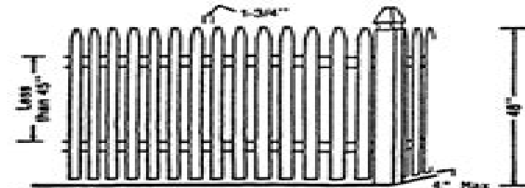
FIG. 1 If Horizontal Members are Less Than 45 in. Apart, Vertical Spacing Shall Not Exceed 1-3/4 in.
