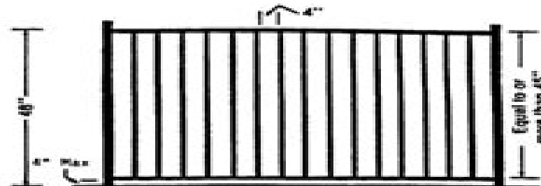
FIG. 2 If Horizontal Members are Equal to or More Than 45 in. Apart, Vertical Spacing Shall Not Exceed 4 in.
