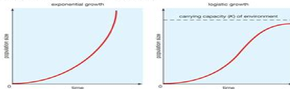
Exponential versus logistic population growth
