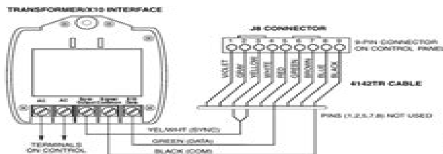
Figure 2. Connections for Vista-40, Vista-50, Vista-128B, Vista-128BP, Vista-250BP, FA1220C, FA1340C, FA1660C, or equivalent
