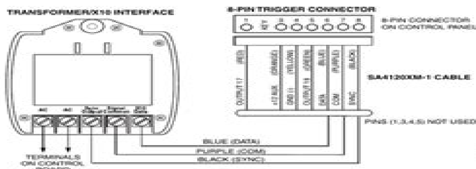
Figure 1. Connections for Vista-15P, Vista-20P, Vista-20PS, FA148CP, FA168C/P/S, or equivalent
