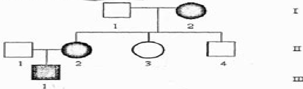
Pedigree showing blue-eyed trait:
