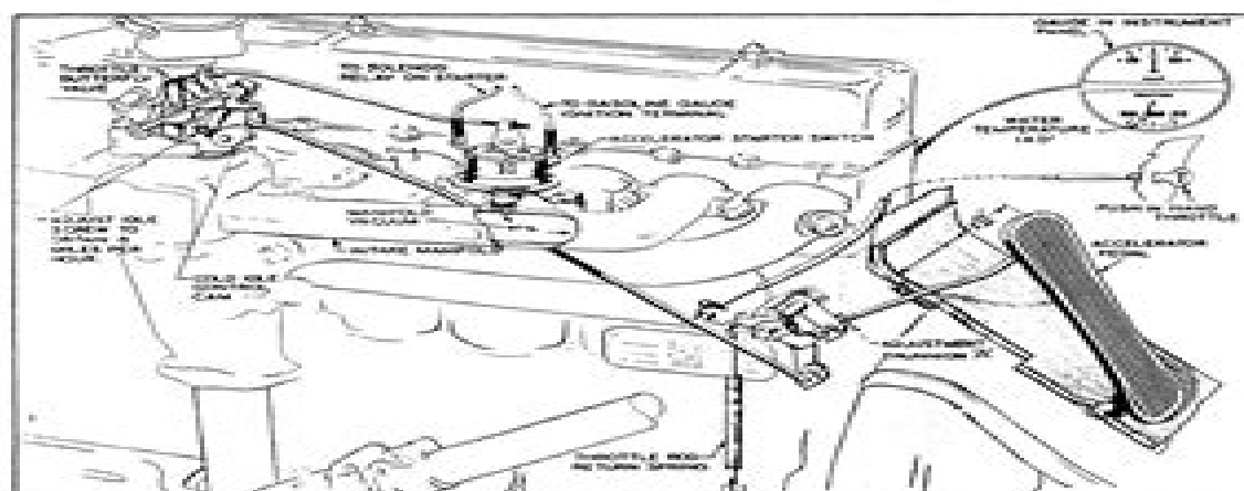
Fig. 119. Diagram—Engine Idle and Accelerator Adjustment
