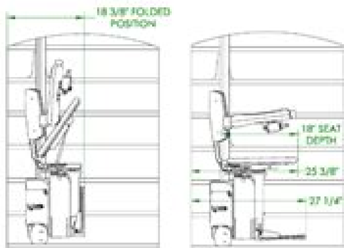
SIDE VIEWS
