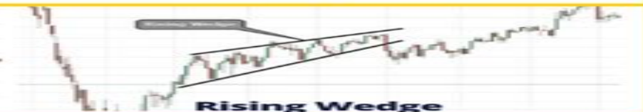
Rising Wedge
