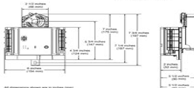
Fig. 1 VAV IP Controller Dimensions
