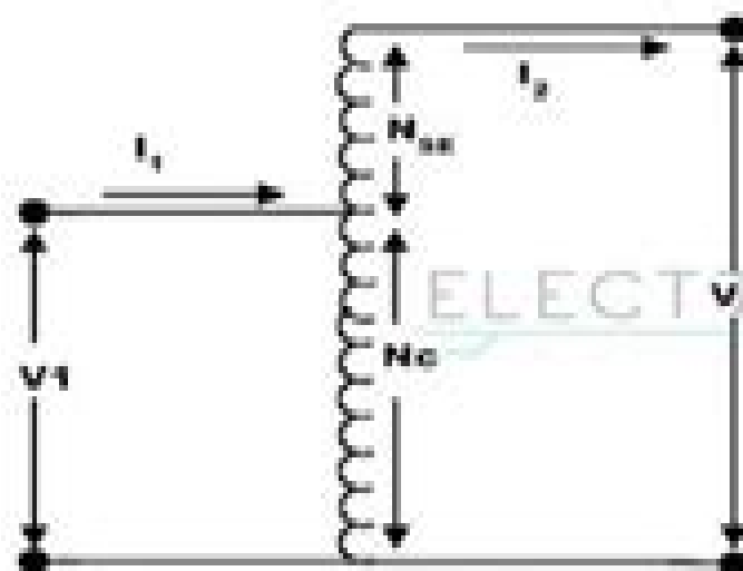
(a) Step up Autotransformer
