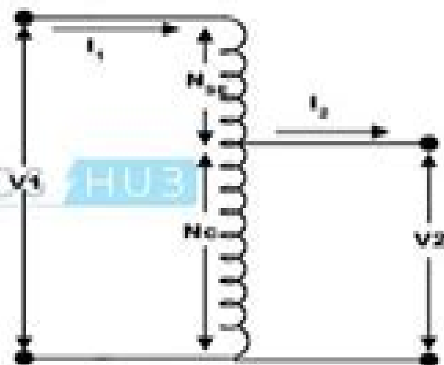
(b) Step down Autotransformer
