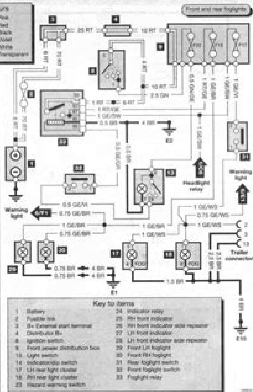
Diagram 3 : Typical hazard/direction indicators and foglights
