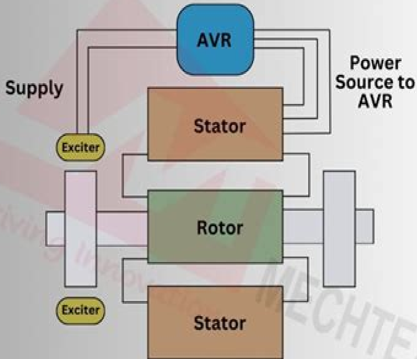
Excitation System of Synchronous Motor
