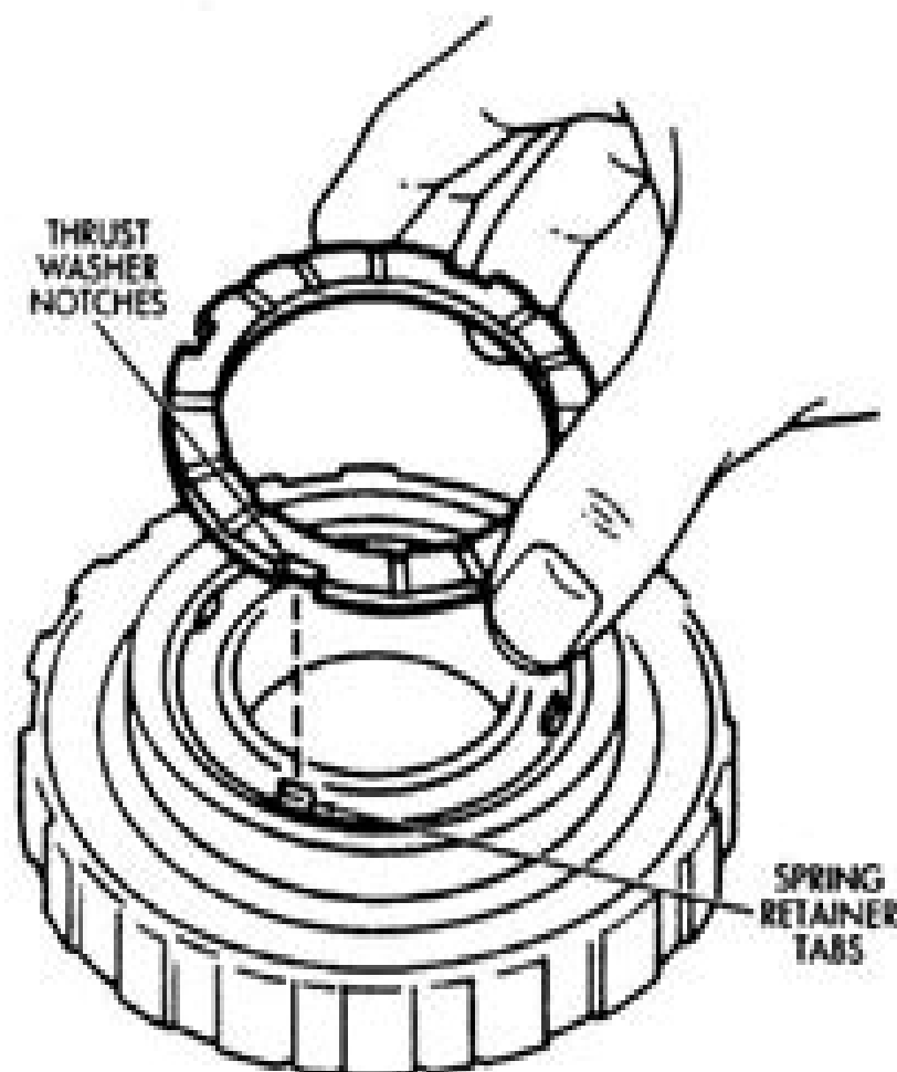
Fig. 8 Installing Thrust Washer
