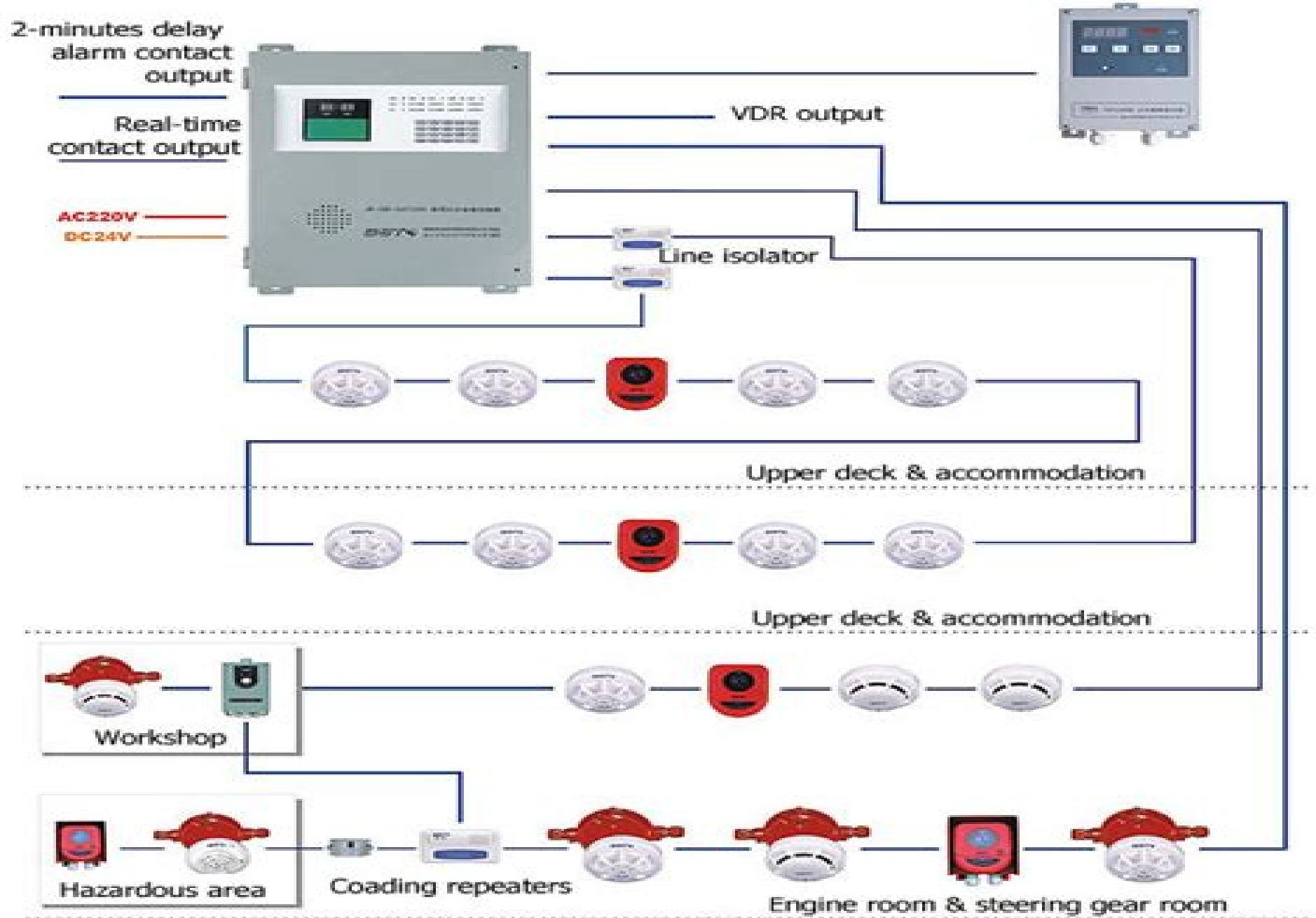
JB-QB-GST200 Fire Alarm System
