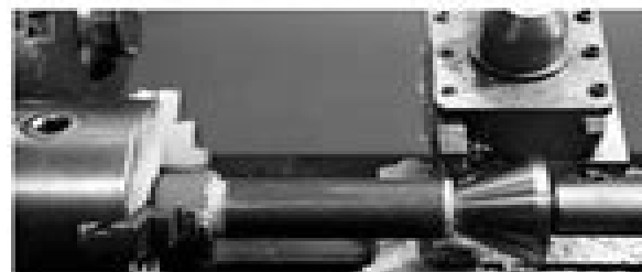
The pipe center in use. Note that, in this case, the pipe has previously been plugged with wood because the pipe is of this soft copper and applying pressure with the center could possibly cause it to bel out.
