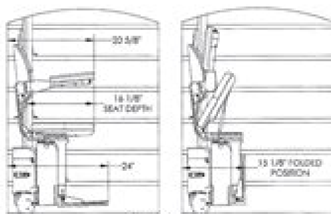
SIDE VIEWS
