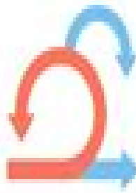
Scrum
