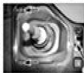
27.4c Two screws at the front (arrowed) and one at the rear (arrowed) secure the selector retaining strap
