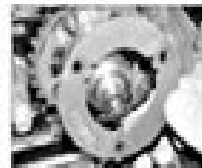
27-17 Undo the three nuts and remove the camshaft cover from the sprocket
