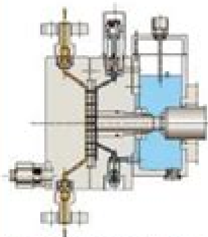
Hydraulic driven Metallic diaphragm with contour plate positioning
