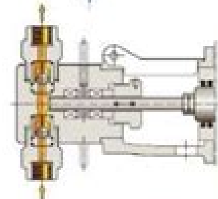
Packed plunger liquid end
