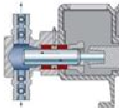
Packed plunger liquid end
