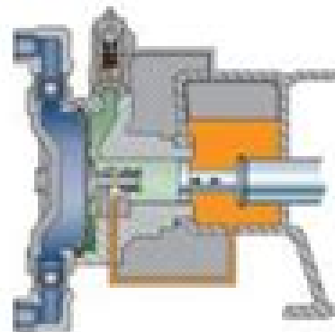
Hydraulic driven diaphragm with diaphragm position valve
