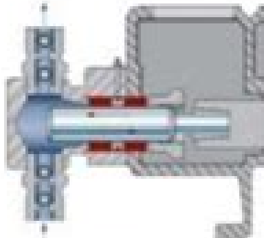
Packed plunger liquid end
