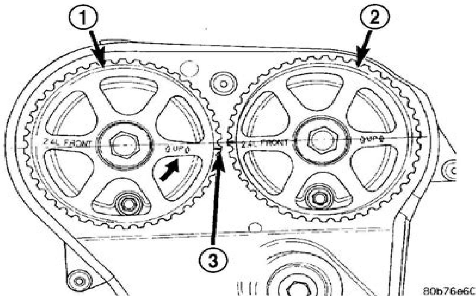
Fig. 84 Camshaft Sprocket Alignment For Timing Belt Installation
