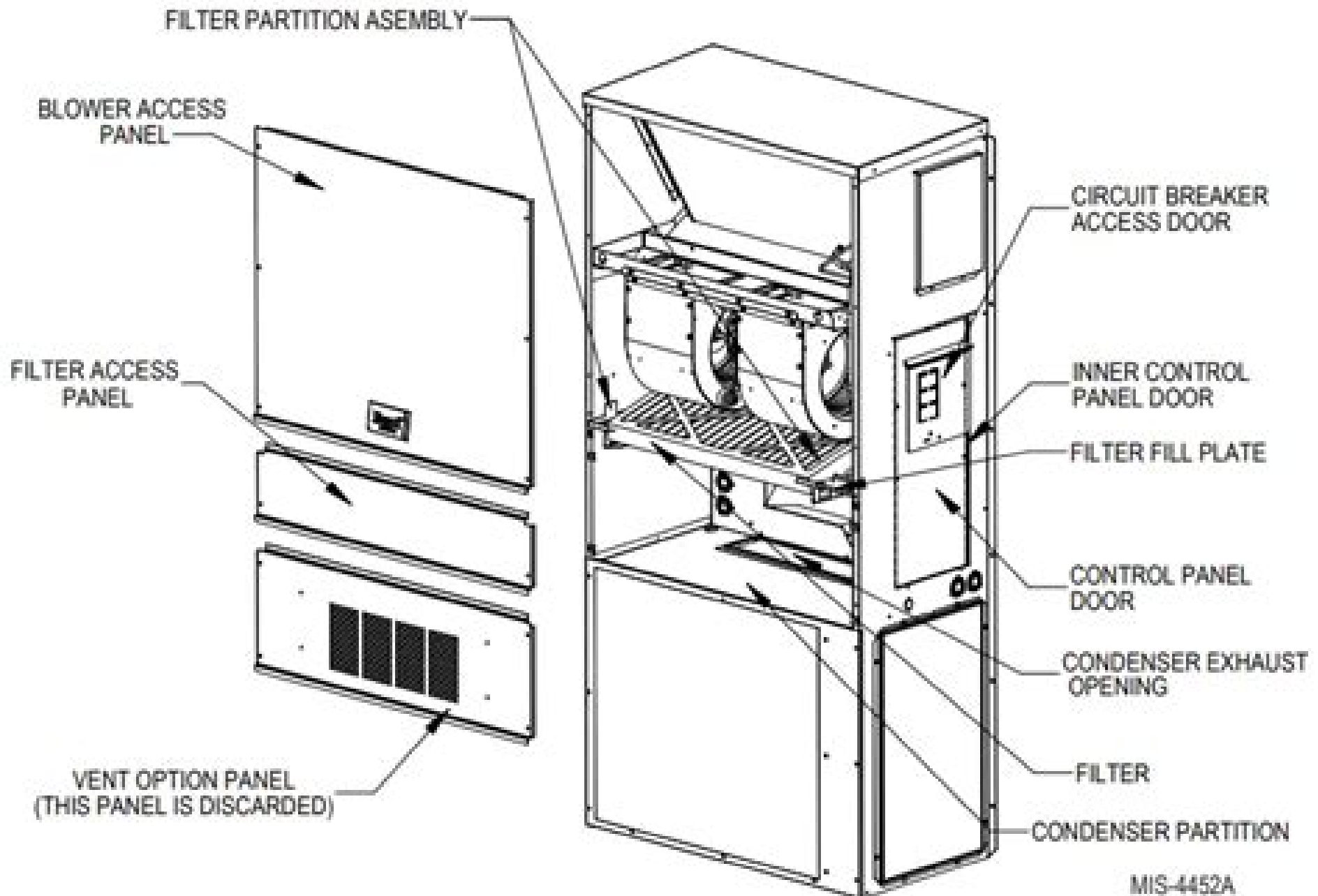
FIGURE 1 Wall-Mount Unit Access Panels
