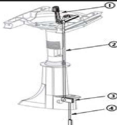
Figure 4 — Gear Selector Operation
