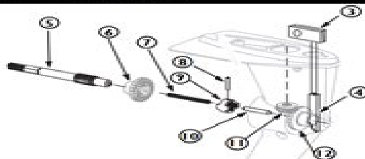
Figure 5 — Forward Gear
