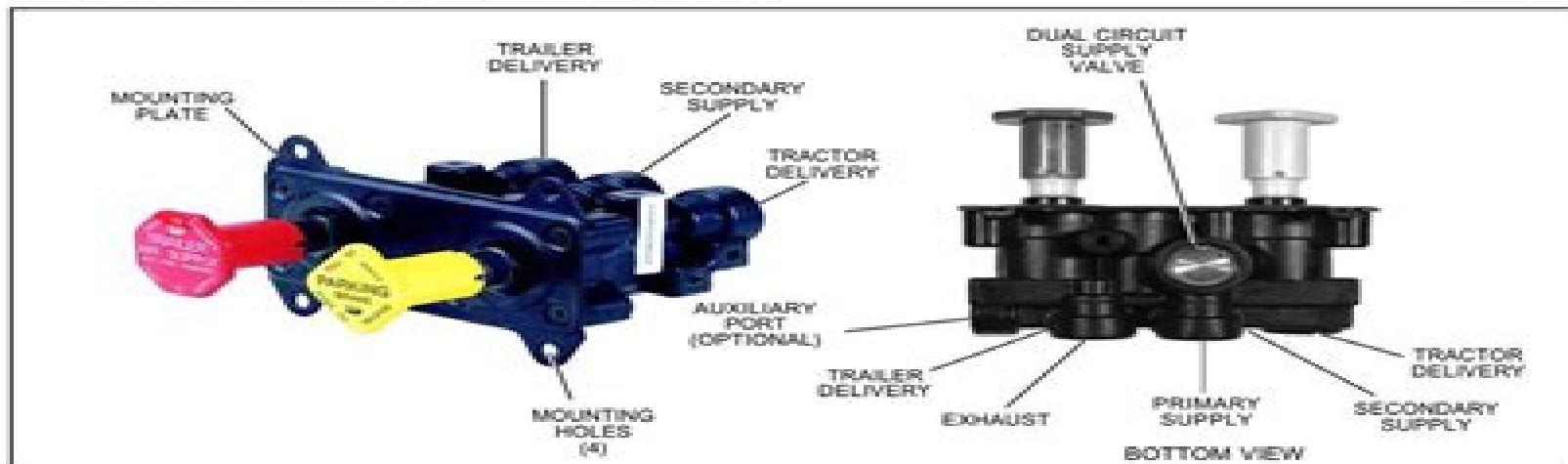
FIGURE 1 - MV-3™ DASH CONTROL MODULE
