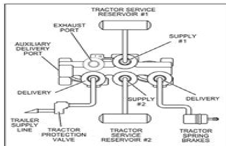
FIGURE 2 - MV-3™ DASH CONTROL MODULE AIR CONNECTIONS
