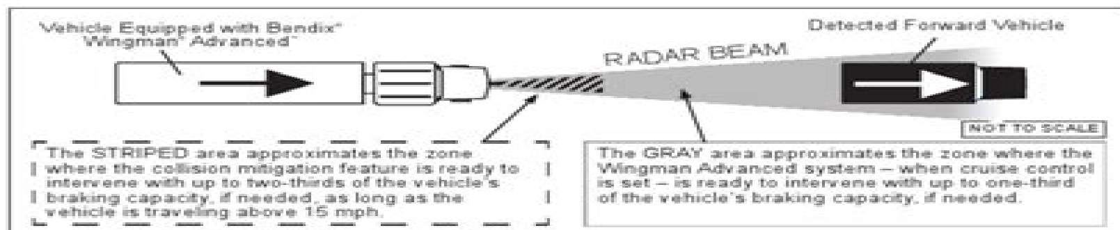
FIGURE 2 - BENDIX® WINGMAN® ADVANCED™ SYSTEM RADAR DETECTION
