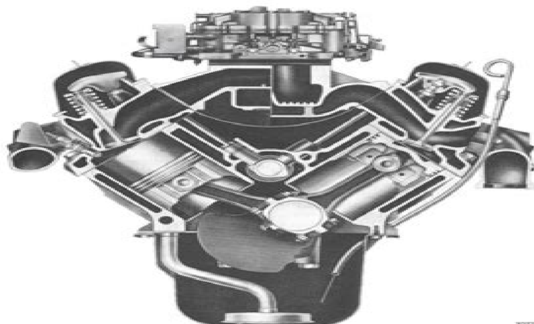
Sectional View of Engine Assembly
