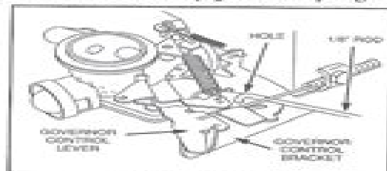
Fig. 4 - Locating Hole
