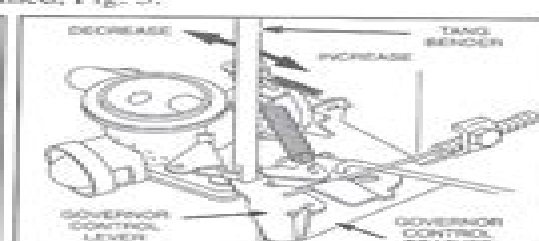
Fig. 6 - Primary Spring Adjustment
