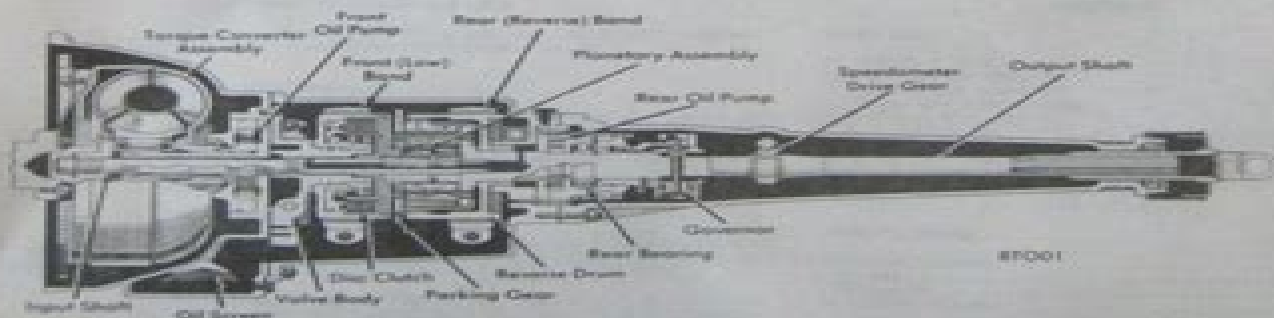
TOYOGUIDE TWO-SPEED TRANSMISSION ASSEMBLY
