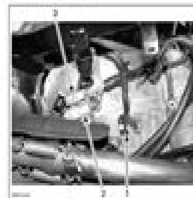
1 Engine pressure switch 2 VSS connector 3 Brake switch connector
