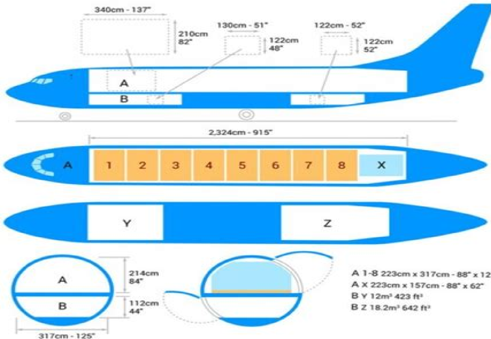
Boeing B737-300F
