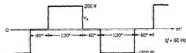
Figure 2. Pulse waveform
