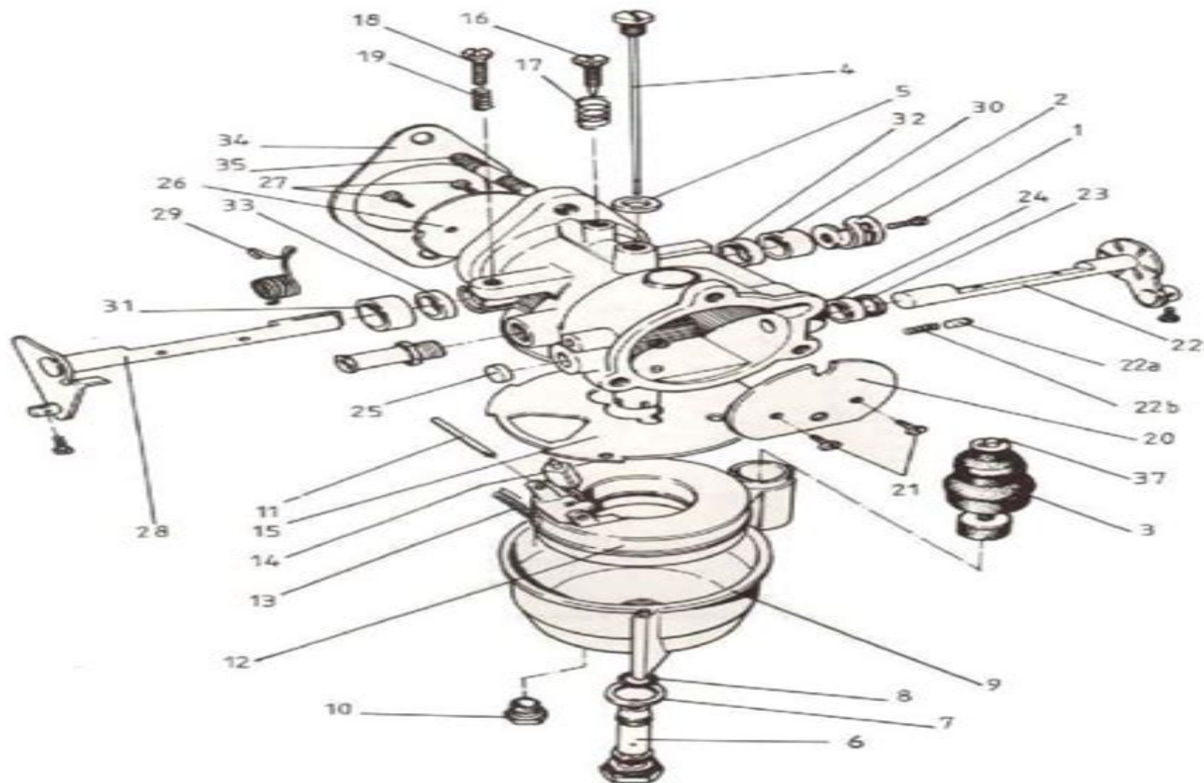
Bendix 16P12 fixed-jet carburettor
