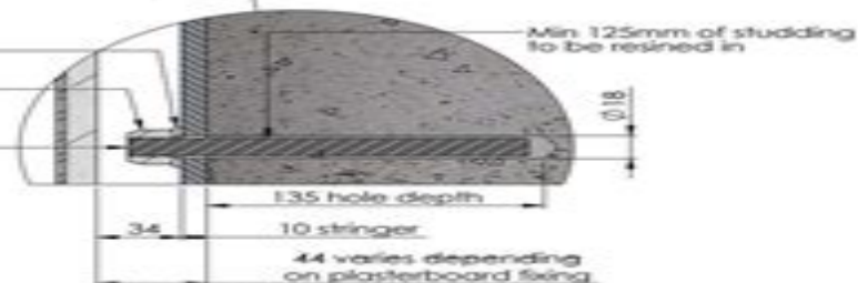
DETAIL C SCALE 2 : 5
