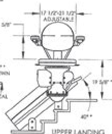
ELEVATION VIEWS
