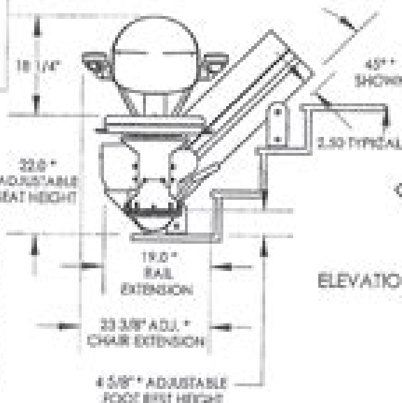
LOWER LANDING
