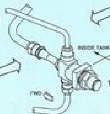
WATER SCAVENGE EJECTOR PUMP
