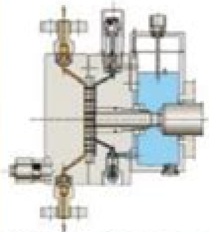
Hydraulic driven Metallic diaphragm with contour plate positioning
