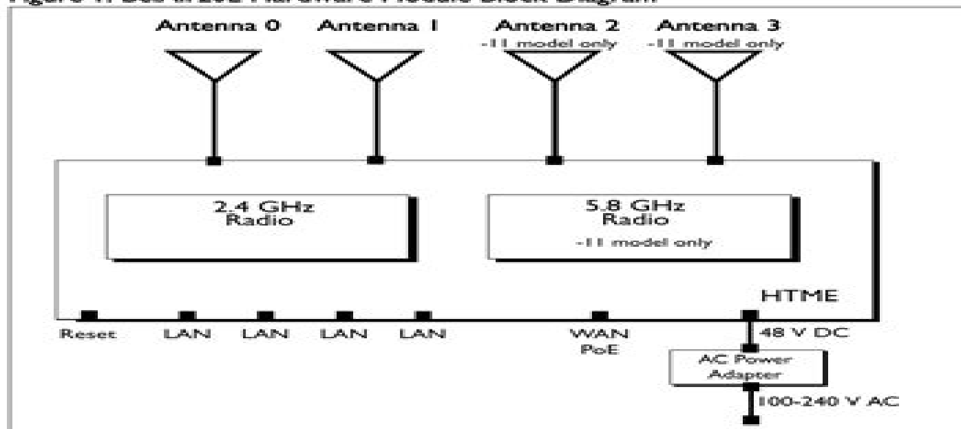
Figure 1: BelAir20E Hardware Module Block Diagram
