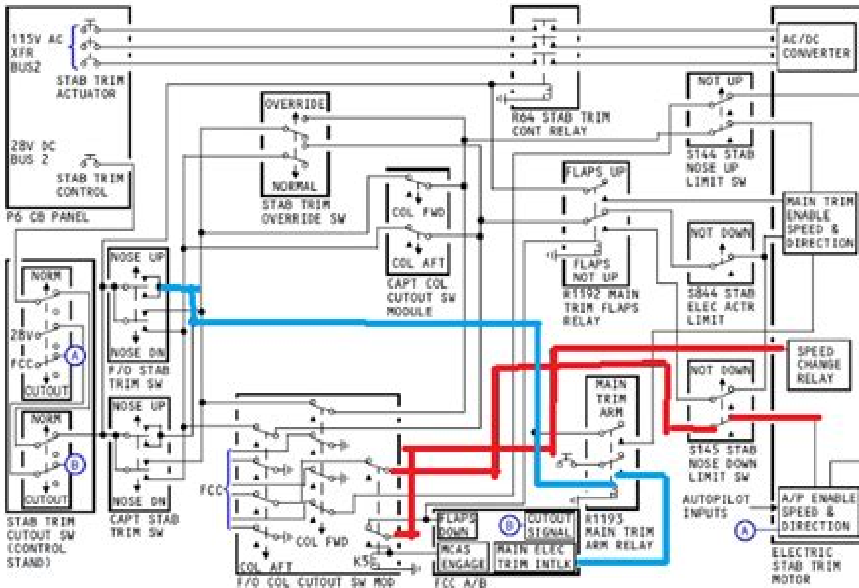
Horizontal Stabilizer Trim Control System - Functional Description - Electric Trim
