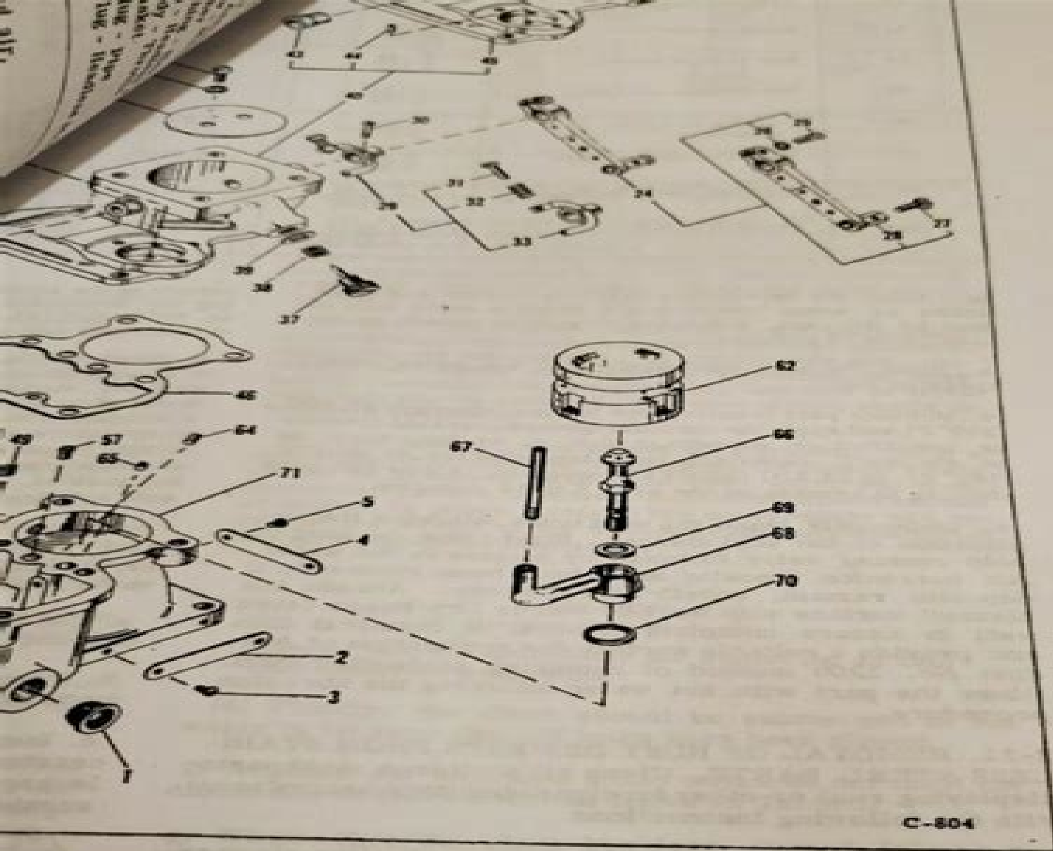
of Stromberg NA-S3A1 Float Carburetor
