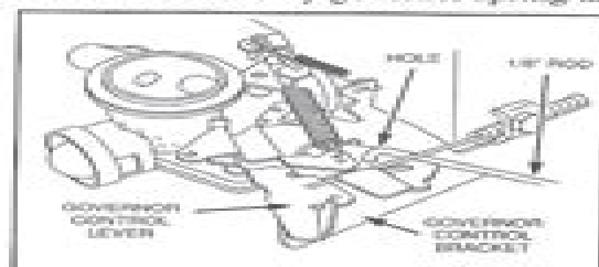
Fig. 4 - Locating Hole
