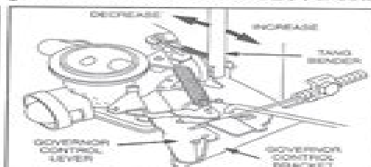
Fig. 5 - Secondary Spring Adjustment
