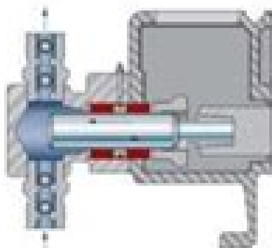
Packed plunger liquid end
