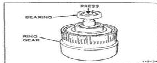
Bearing Installation
