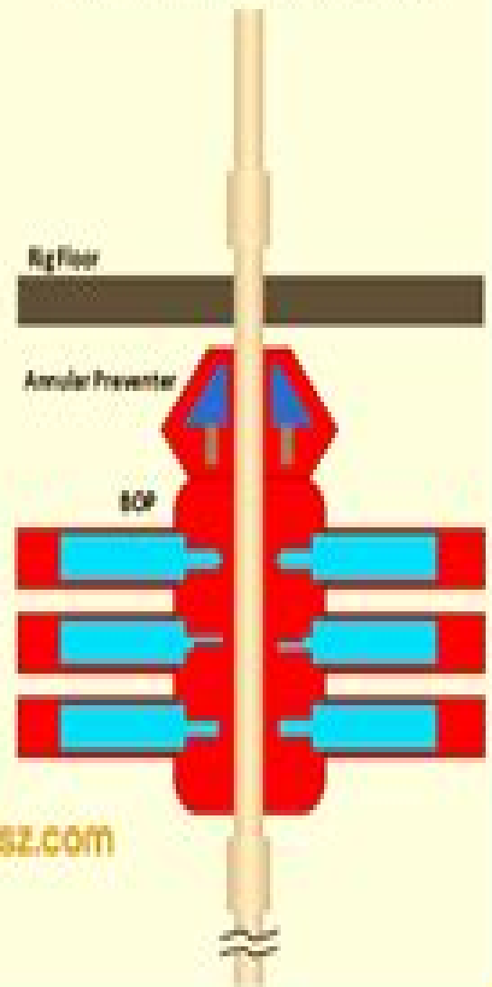
(B) Cut-away Side View of BOP (Drill Pipe Space Out)
