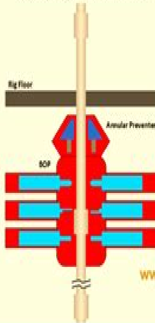
(A) Cut-away Side View of BOP (Drill Pipe not Space Out)
